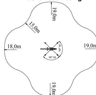
Basket load 100 kg
